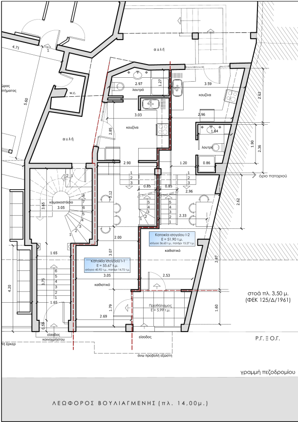
Ground Level
